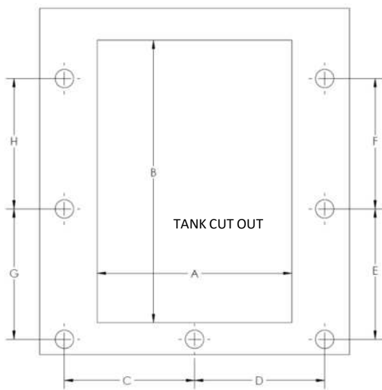
Details for side mounting FB/FBN 700 SM 40
